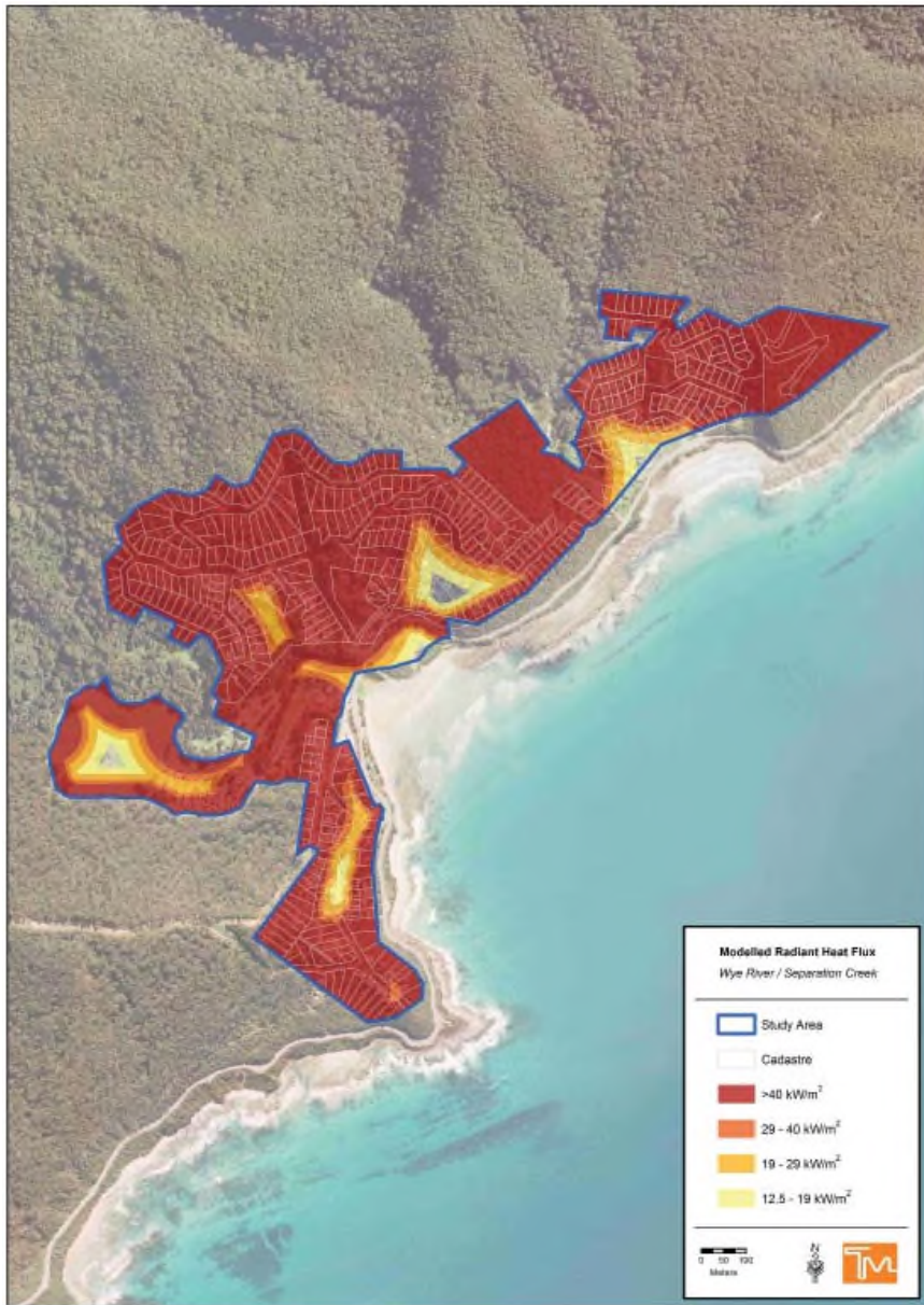
Map 26: Wye River / Separation Creek - Radiant Heat Flux
